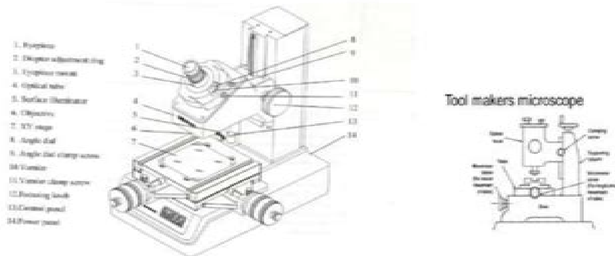
Figure 10: Tool Makers Microscope
