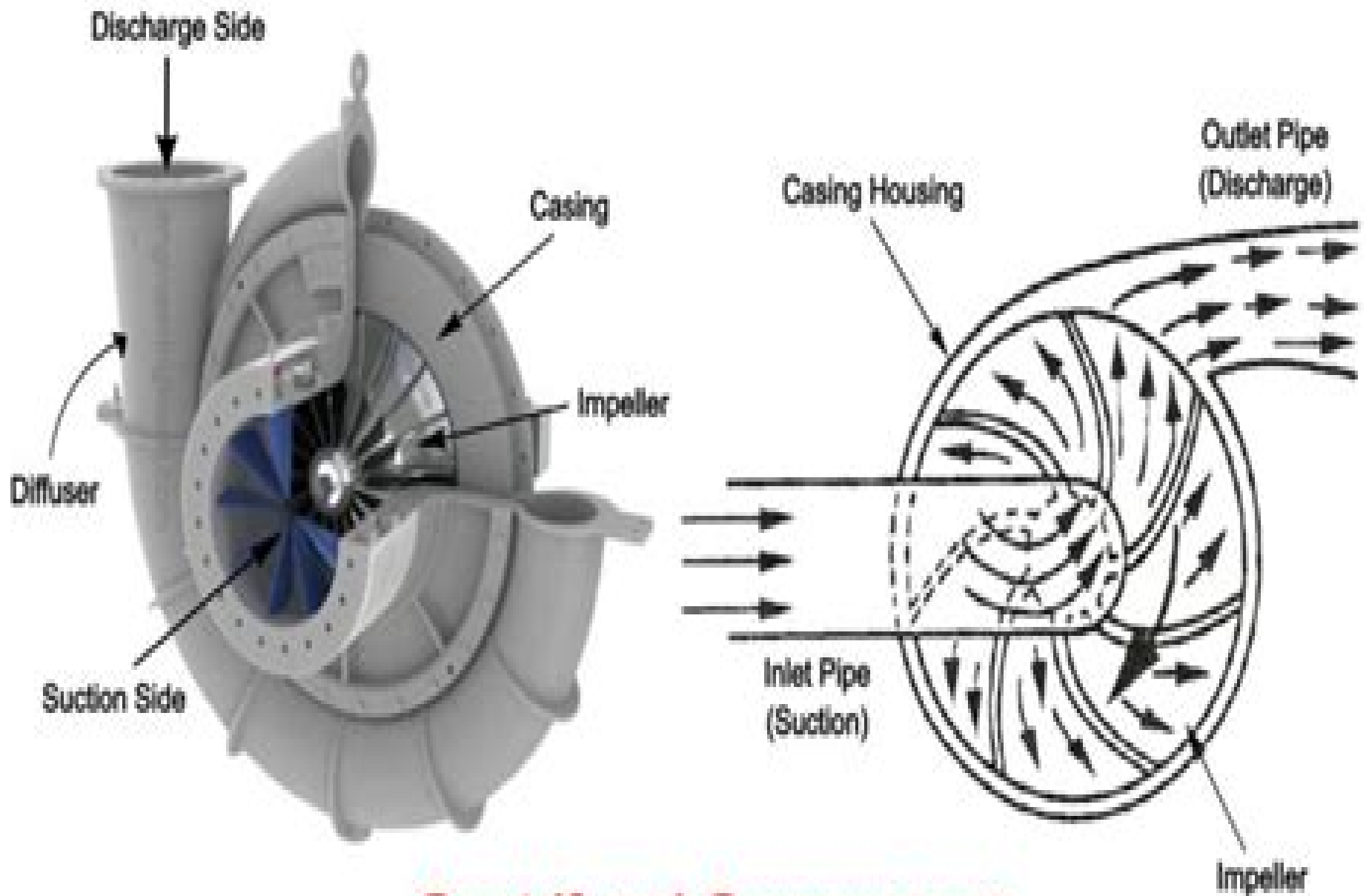
Centrifugal Compressor
