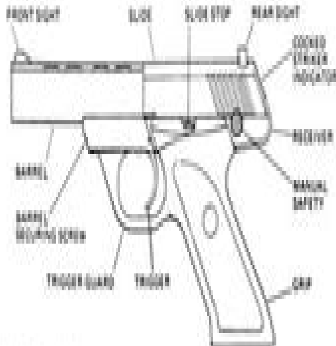
FIGURE 1. COLT ® 22 PISTOL
