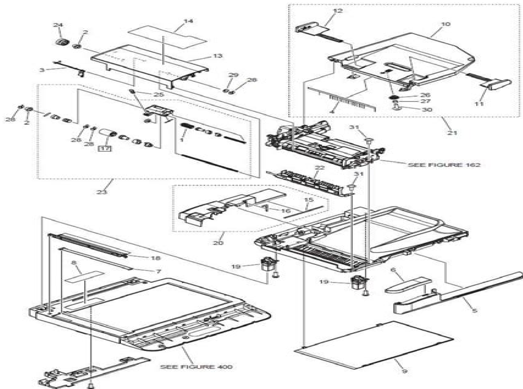
FIGURE 160 READER/ADF ASSEMBLY
