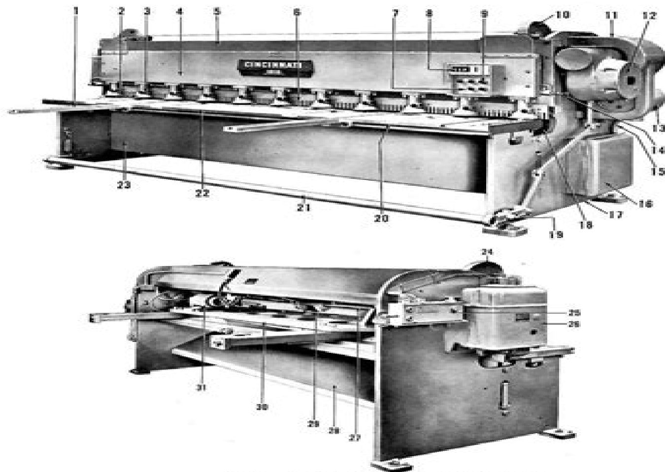
Fig. 1. Identification 10 Series Shears
