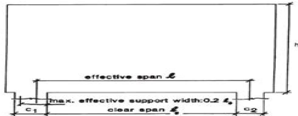
Figure 1.2 CIRIA Guide 3—meanings of symbols c_1 , c_2 , h , l and l_s
