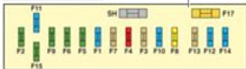
Fusebox C
