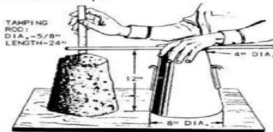
Figure 2: Slump measurement
