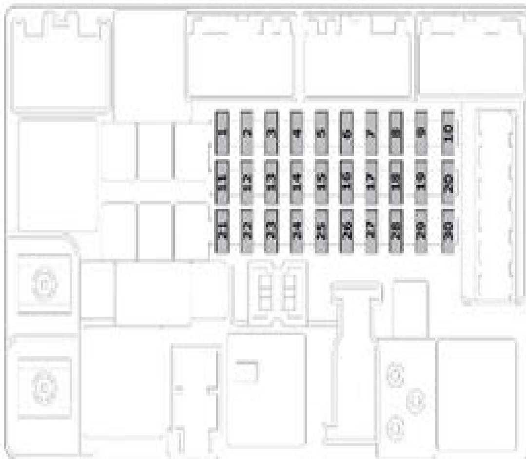
Left-side A-pillar fuse box diagram
