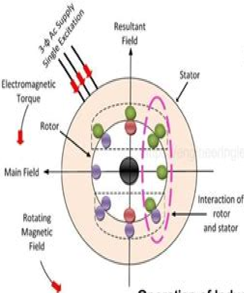
Operation of Induction Motor
