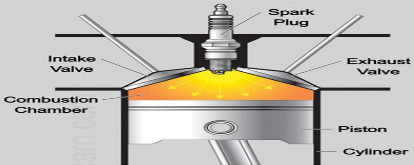
(a) Normal Combustion
