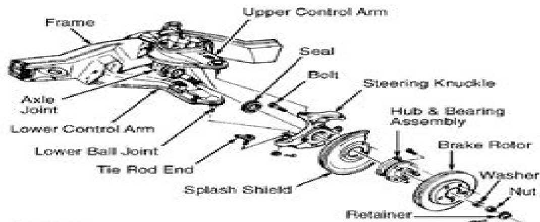
Fig. 1: Exploded View Of Hub & Steering Knuckle Assembly ("T" Series Shown; "K" & "L" Series Are Similar)
