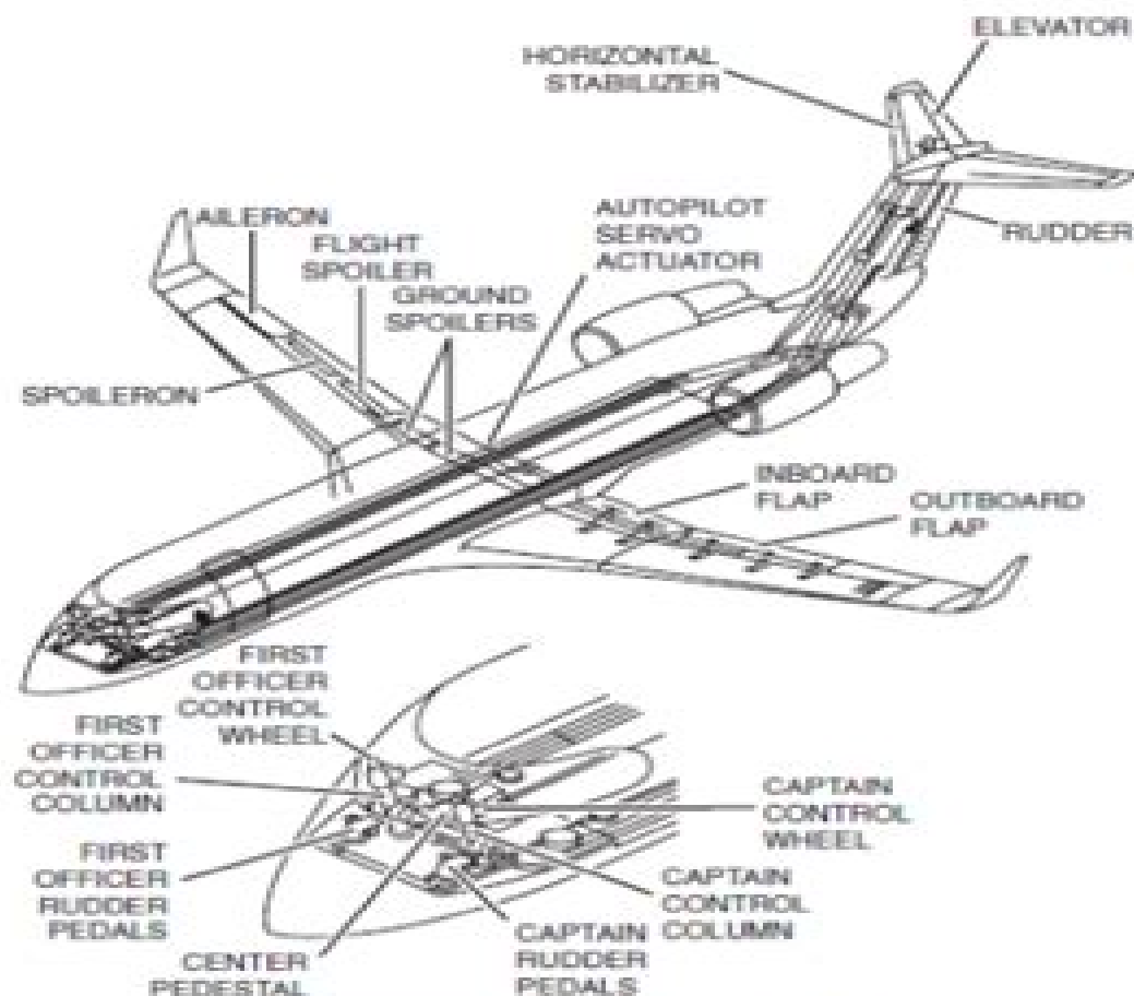
Figure 1-46 Flight Controls
