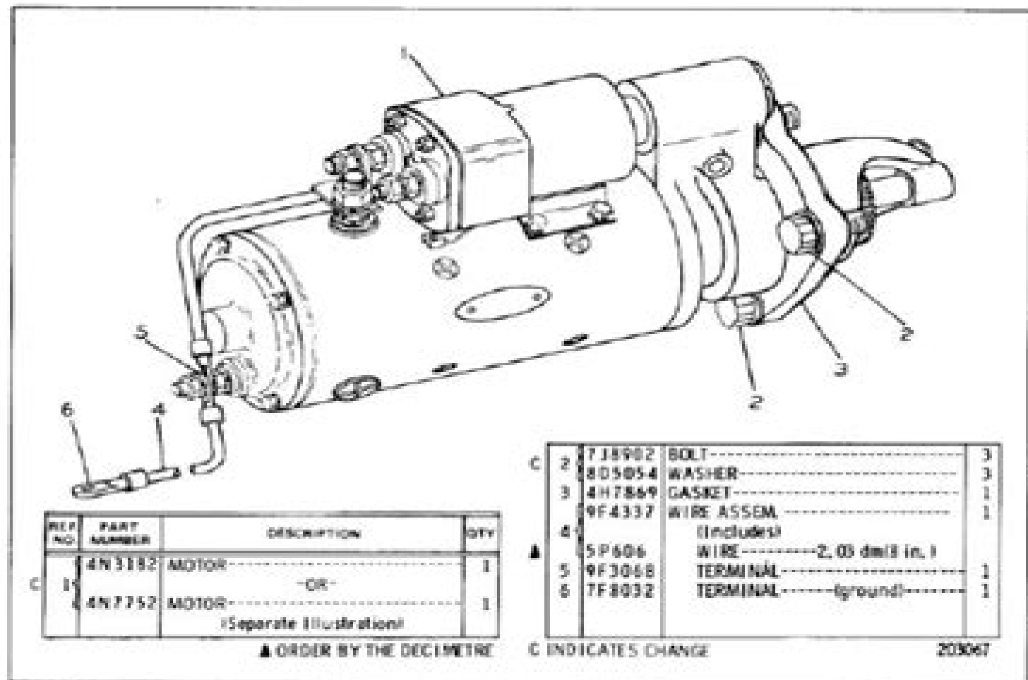
7S3822 ELECTRIC STARTING MOTOR GROUP—24 Volt—Type 2 Part of 1P4433 Direct Electric Starting Arrangement listed on Page 21. 4N3182 and 4N7752 Motor parts are shown on Pages 23, 24, 25, 27A and 27B AN ATTACHMENT
