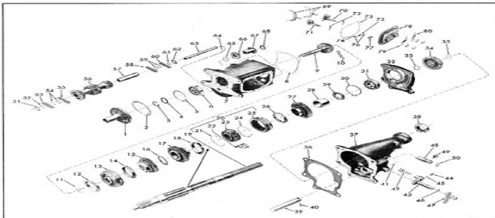
Fig. 55 4-Speed Transmission-Exploded View
