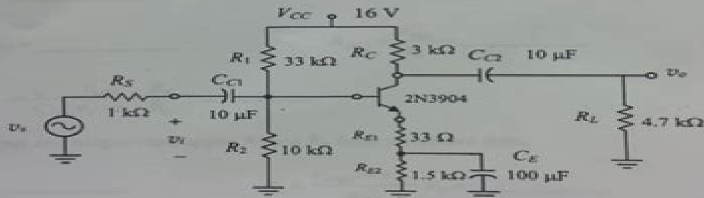
Figure 6: Common-emitter amplifier.
