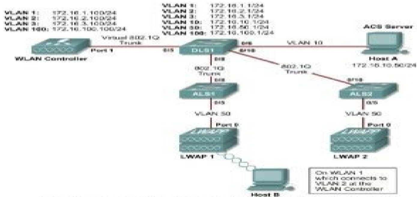
Figure 1-1: Ethernet Connectivity Diagram for Module 6, External WLAN Controller
