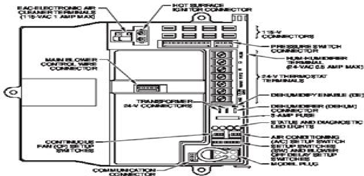
Fig. 12— Variable-Capacity Control Center
