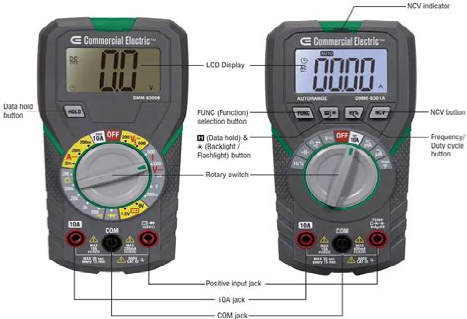
DMM-8300B
