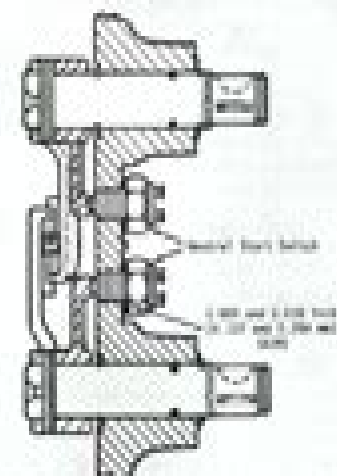
Fig. 38—Cross-sectional view showing neutral start switch plate placement and shift shims. Refer to text.
