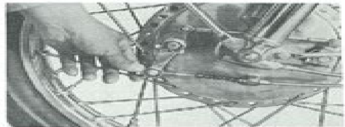
Fig. 11-11-2 Adjusting front brake
