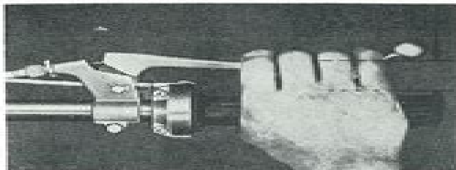
Fig. 11-11-1 Front brake lever play
