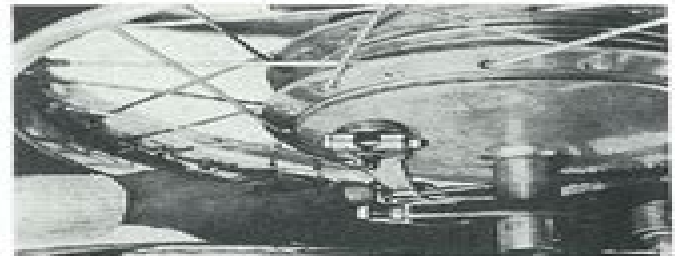
Fig. 11-11-4 Adjusting rear brake
