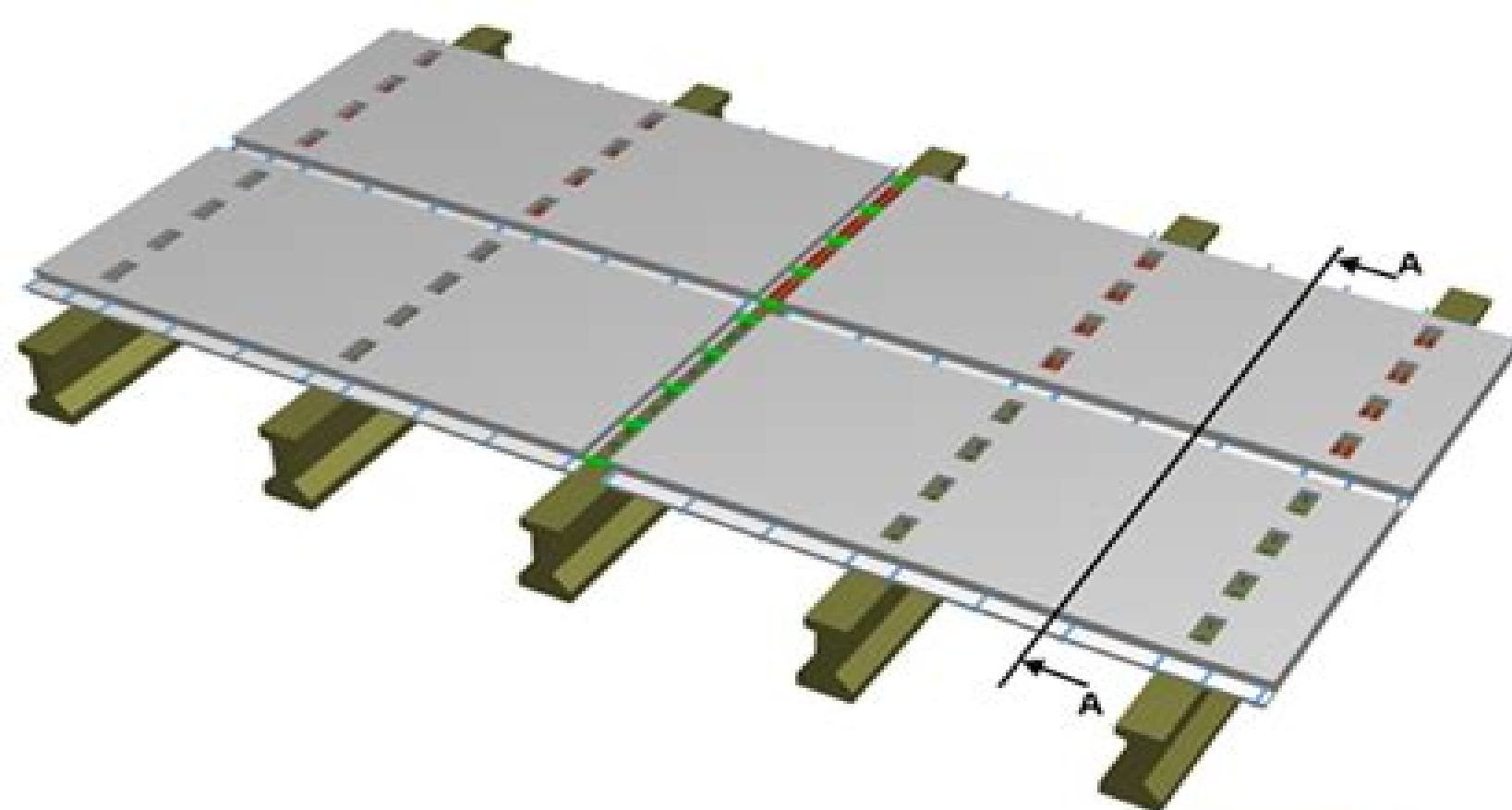
a) Schematic of a bridge with UHPC waffle panel
