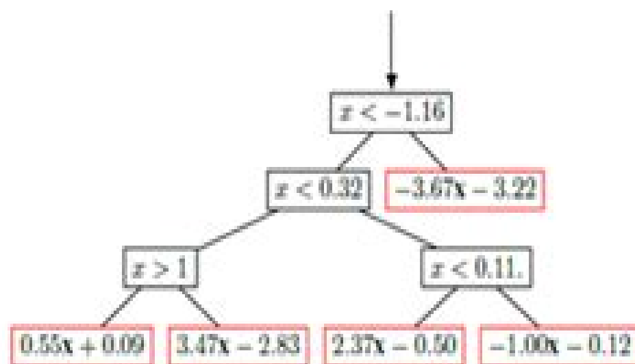
(a) Cleared Tree
