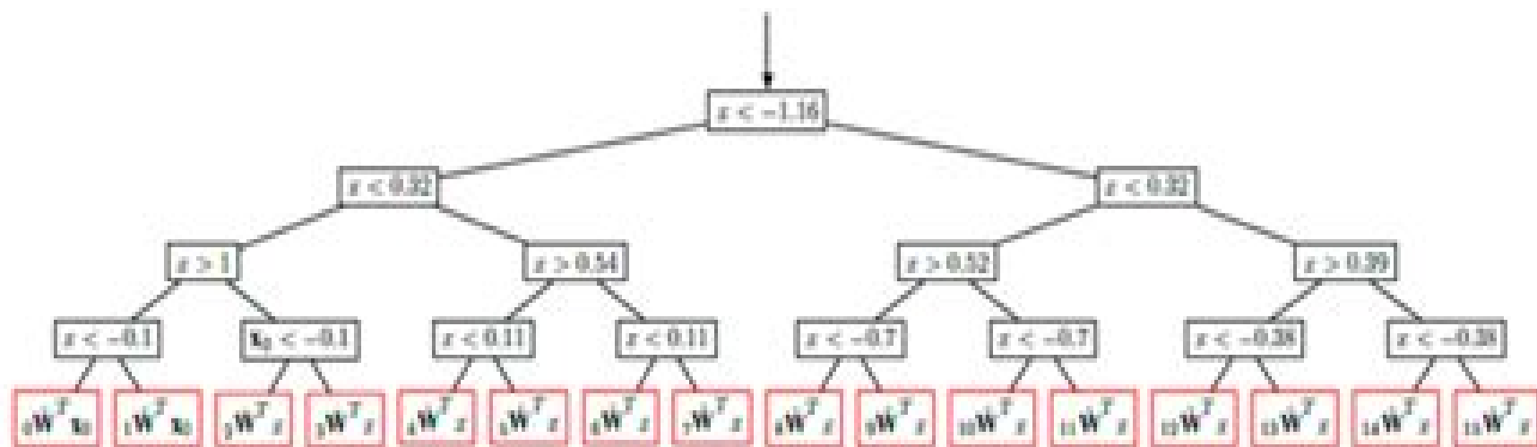
Figure 2. Decision Tree for a y = x^2 Regression Neural Network
