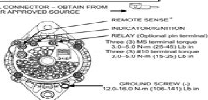
FIGURE 2 - 24SI™ (4-Terminal studs & 3-Terminal studs & Pin)
