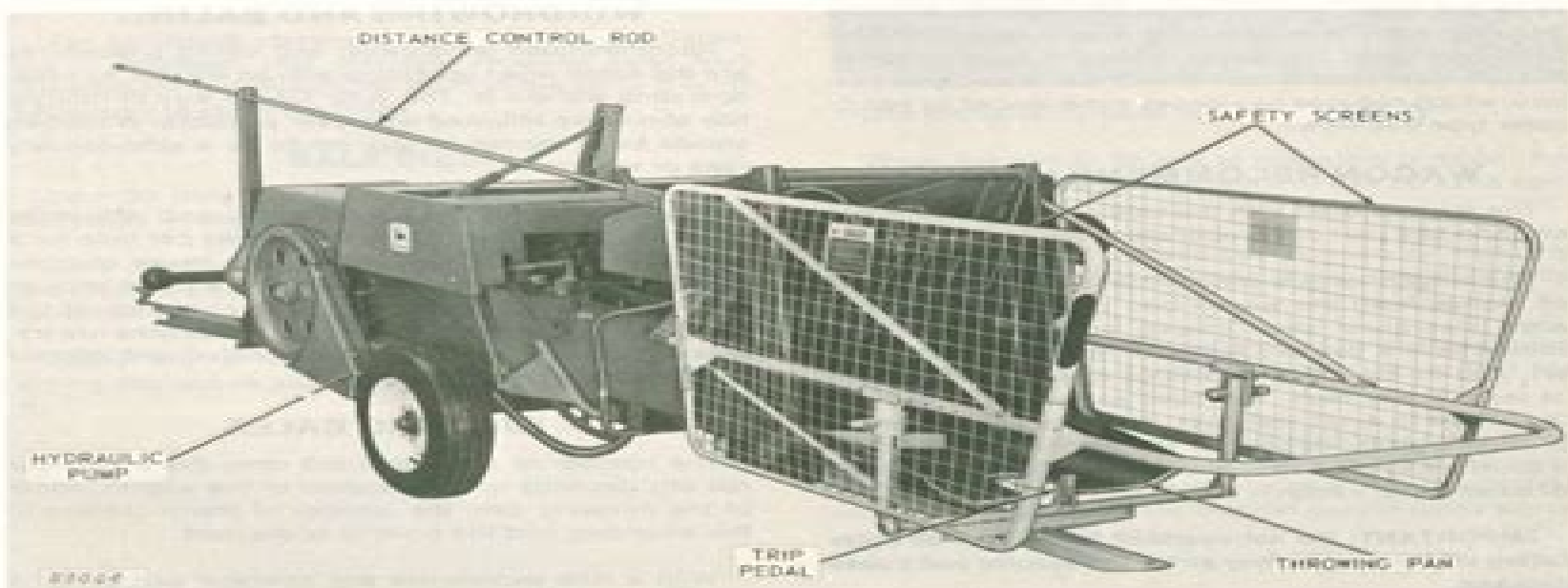
John Deere 30 Bale Ejector on 336 Twine Baler
