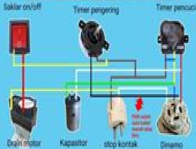
Diagram mesin cuci otomatis jadi manual
