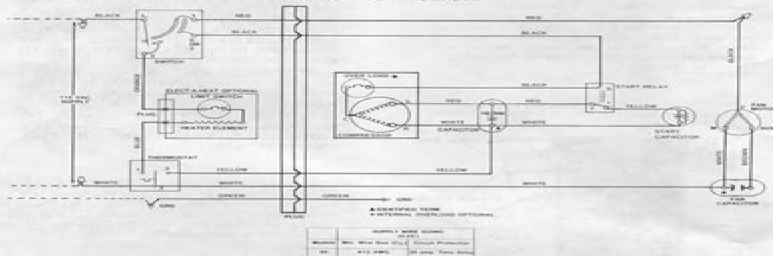
LATCHED TYPE WIRING DIAGRAM
