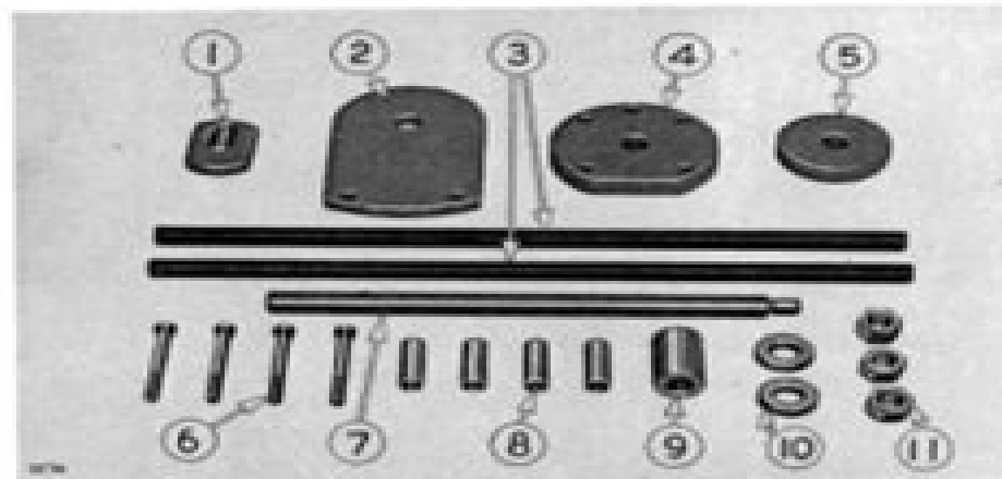
FIG. 1. FLANGE-TYPE PUMP HOUSING CAMSHAFT BUSHING PULLING AND REPLACING TOOLS
