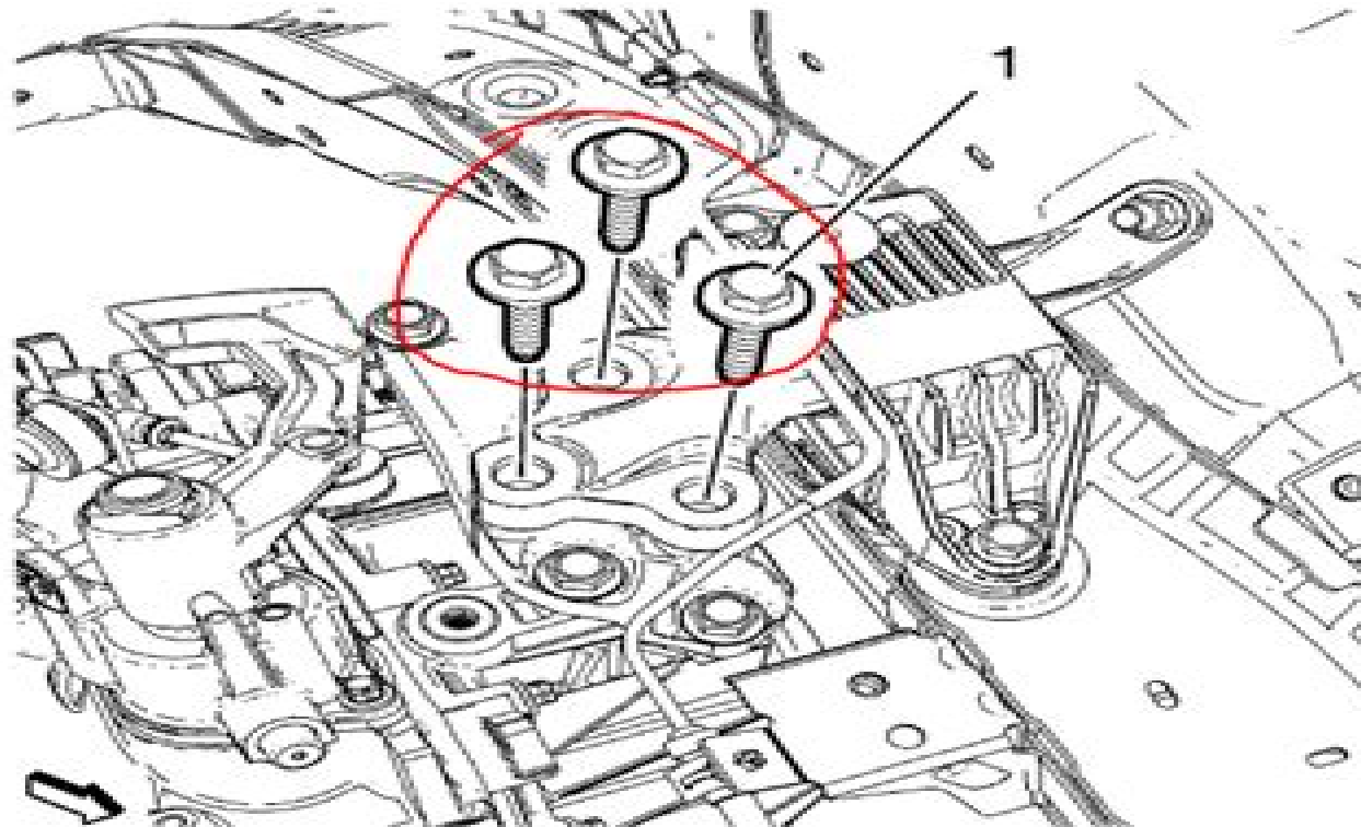
Fig. 80: Transmission Mount Bolts Courtesy of GENERAL MOTORS COMPANY
