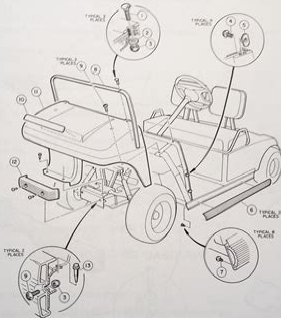
Figure 5-10 — Front Body Removal
