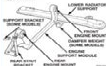
Fig. 17 Engine Support Module
