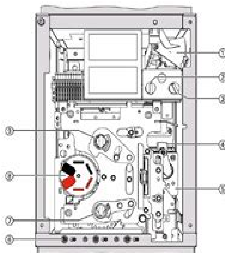
Fig. 5: Front operating mechanism in ring-main feeder
