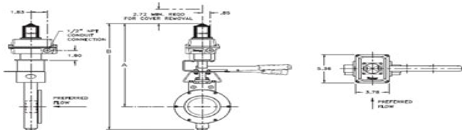
Figure 1. Wafer Valve (3" Valve Pictured)
