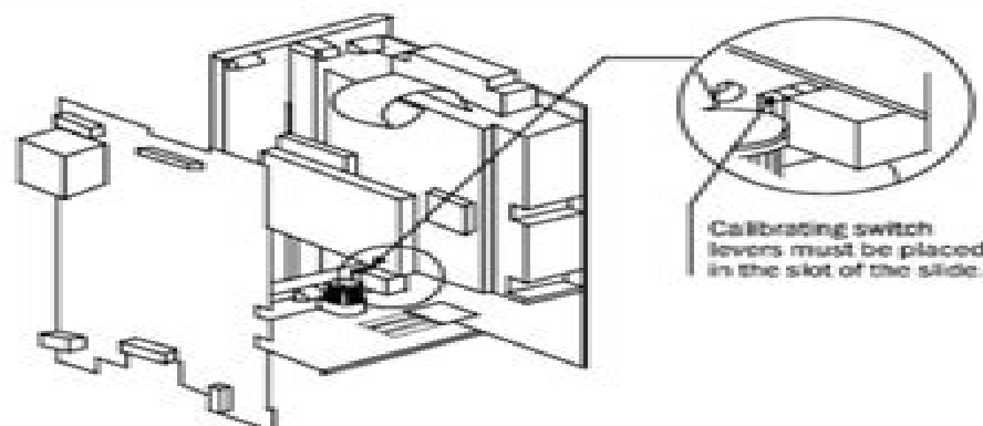
Figure 7-4. Calibration switch
