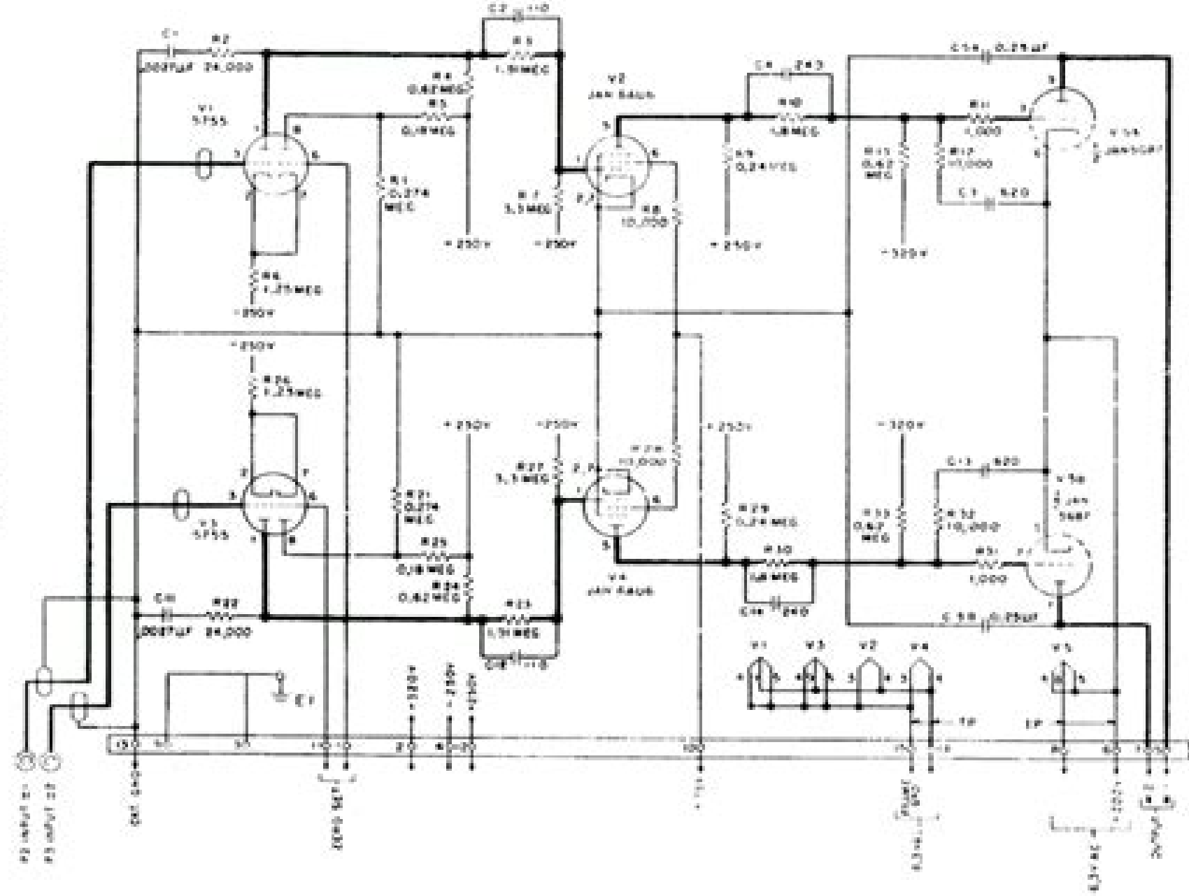
Figure 2. D-153844: DC Amplifier
