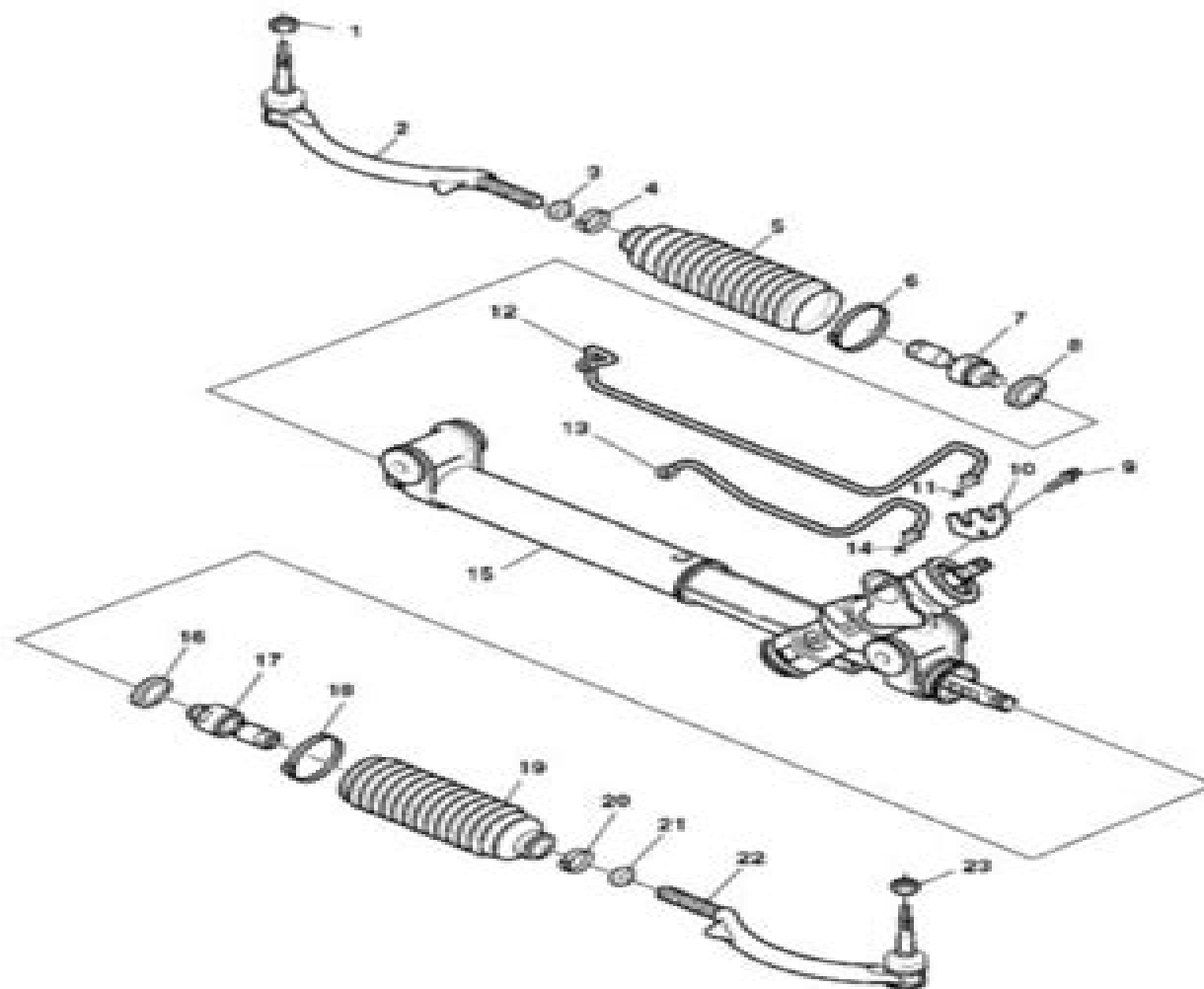
Fig. 1: Identifying Power Steering Gear Components Courtesy of GENERAL MOTORS CORP.
