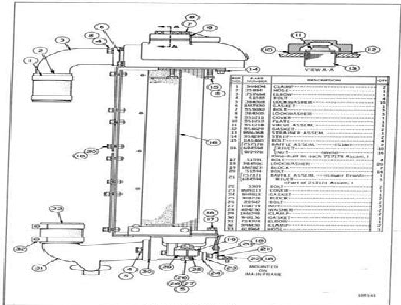
RADIATOR—Side View Refer also to Page 135 for special parts
