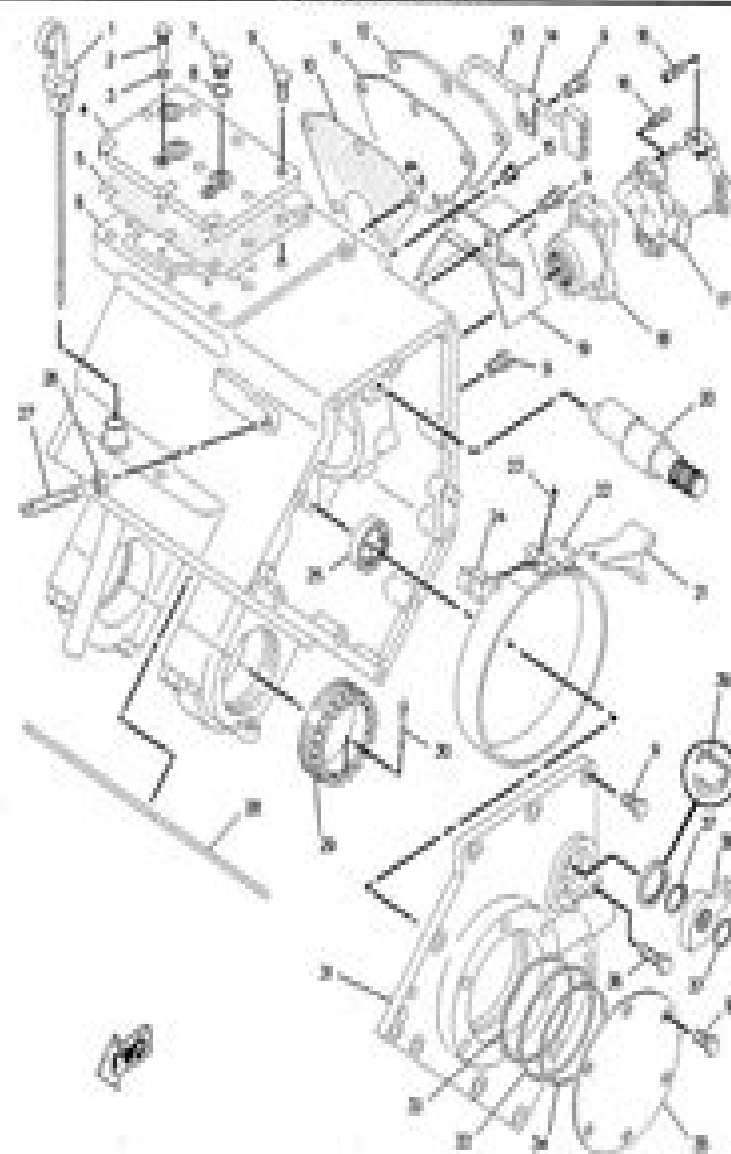
STEEL CASE & PARTS OF TRANSMISSION Type 2-57H 2NCT-67H, 4NCT-70H, 4NCT-87H, 8NCT-400
