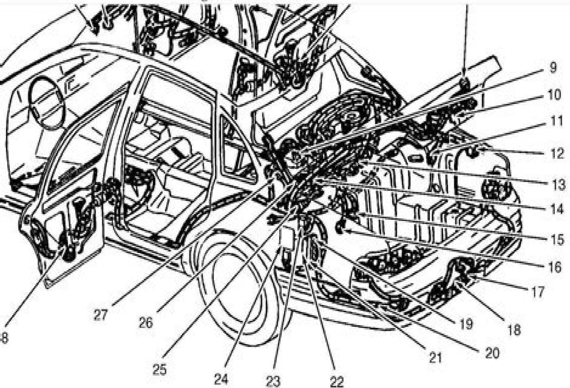
Fig. 5: Vehicle Overview
