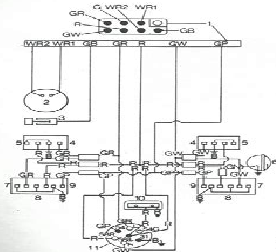
Figure H147 REAR HARNESS
