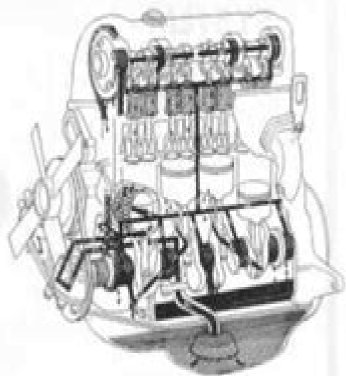
Fig. EL-1 Lubricating circuit
