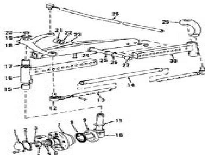
Fig. 2—Exploded view of Model 885N front axle, wheel spindle, hub and bearing assembly. Note shims (5) used to adjust bearings.
