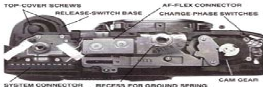
FIG. 2 BOTTOM VIEW
