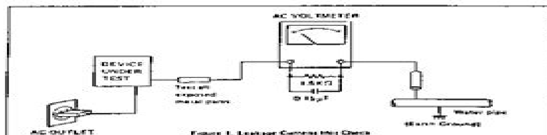
Figure 1. Leakage Current Hot Check
