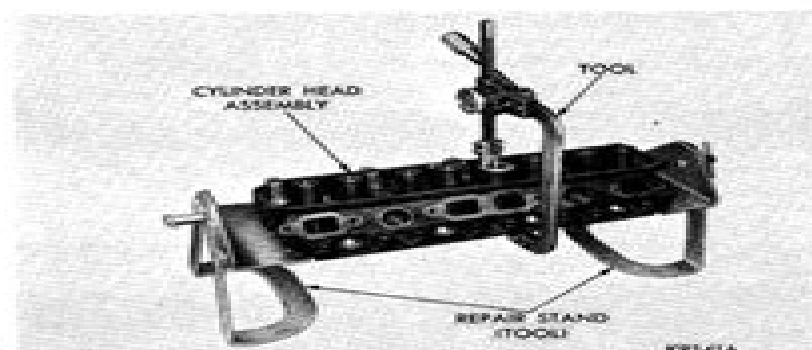
Fig. 6—Compressing Valve Spring
