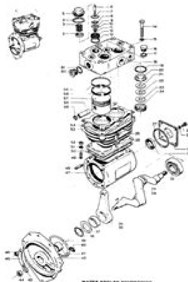
WATER-COOLED-COMPRESSOR Type TR 42 140 DAF no. 28894
