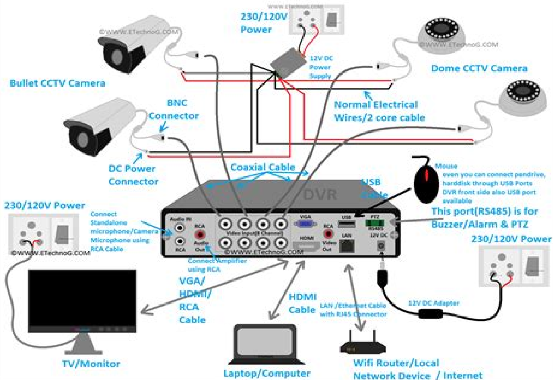
Figure. 01 CCTV Camera Wiring Diagram for Installation with DVR
