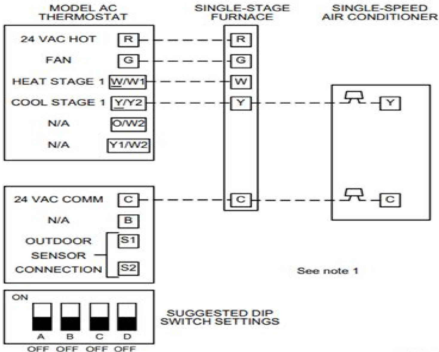
→ Fig. 2—Single-Speed Air Conditioner with Single-Stage Furnace—Model AC Thermostat
