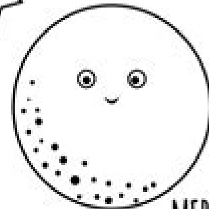
MERCURY
