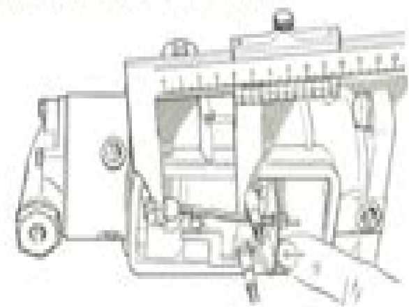
Fig. 2 Measurement of governor link length
